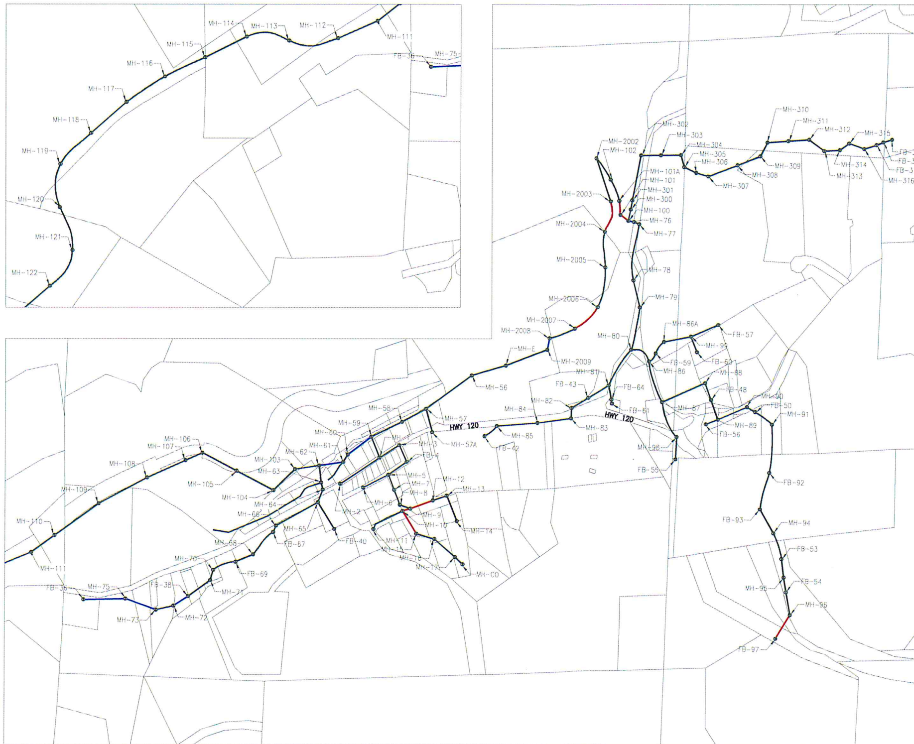
FIGURE 4-2 ALTERNATIVE II GROVELAND SEWER MAINS TO BE REPLACED/REHABILITATED
